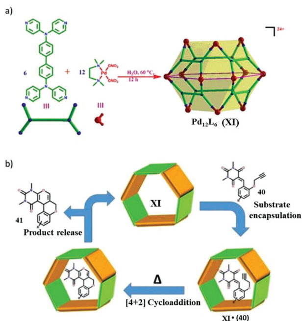
Fig. 52 (a) Synthesis of orthobicupolar \text{Pd}_{12} cage XI. (b) Proposed pathways for the intramolecular hetero Diels–Alder reaction of 40 within cage XI. Reproduced with permission from ref. 154. Copyright 2018, John Wiley & Sons, Ltd.
