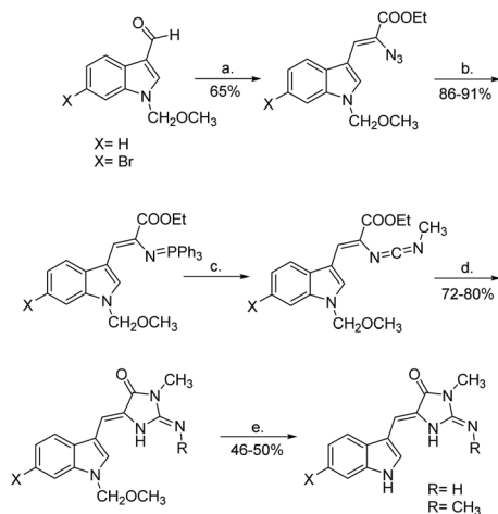
Scheme 30 Iminophosphorane-mediated ring formation to produce (Z)-aplysinsopins. Reagents: (a) \text{N}_3\text{CH}_2\text{COOC}_2\text{H}_5 , NaOEt, EtOH, -15\text{ }^\circ\text{C} , (b) \text{PPh}_3 , \text{CH}_2\text{Cl}_2 , rt, (c) \text{CH}_3\text{-NCO} , toluene, rt, (d) \text{NH}_2\text{R} , toluene, 45\text{ }^\circ\text{C} , (e) \text{HCOOH} , reflux.
