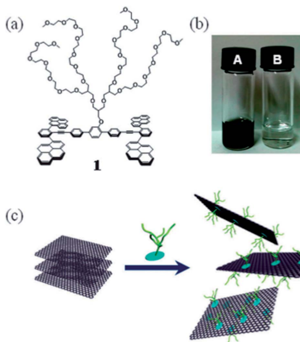
Fig. 13 Exfoliation process of graphite and stabilization of graphene through the \pi - \pi interaction with tetrapylene derivative. This figure has been reproduced from ref. 91 with permission from R. Soc. Chem. , Copyright 2016.
