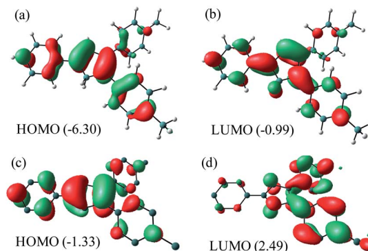
Fig. 5 HOMO and LUMO of \text{Me}_2\text{Cp-H} (1) (a and b) and \text{Me}_2\text{Cp}^- anion (c and d) calculated at M06-GD3/def2TZVP level of theory (in gas phase). Energies are in eV.
