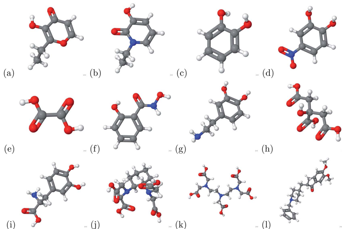
Fig. 3 The chelators above were used in the current study. (a) 2-Ethyl-3-hydroxypyrr-4-one, (b) 1-ethyl-3-hydroxypyridin-2-one, (c) catechol, (d) 4-nitro-catechol, (e) oxalic acid, (f) salicylhydroxamic acid, (g) dopamine, (h) citric acid, (i) L-Dopa, (j) CDTA, (k) DTPA and (l) donepezil. For the atomic structure, the carbon, hydrogen, oxygen, nitrogen, and aluminum atoms are represented by gray, white, red, blue, and grayish red respectively.
