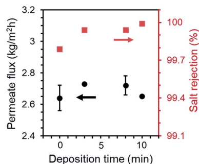
Fig. 5 Permeate flux and salt rejection of 0.45 \mu\text{m} PP membranes after PHDFA coating with varying deposition time. Test condition: feed temperature at 50^\circ\text{C} , flow rate at 0.81\text{ L min}^{-1} , NaCl concentration at 30\text{ g L}^{-1} .
