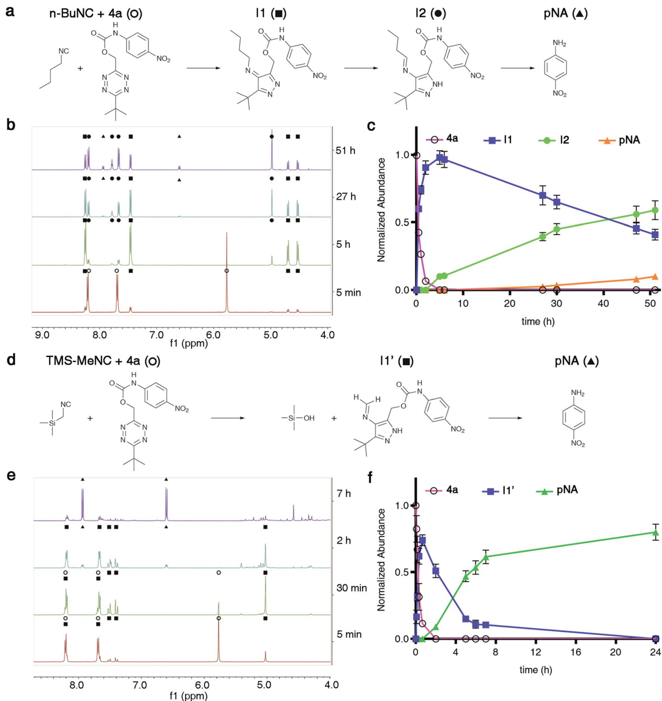
Fig. 4 ^1\text{H-NMR} analysis of reactions between isonitriles n\text{-BuNC} or \text{TMS-MeNC} and 4\mathbf{a} to liberate \mathbf{pNA} . (a and d) Proposed intermediates in the reaction between n\text{-BuNC} (a) or \text{TMS-MeNC} (d) and 4\mathbf{a} leading to the release of \mathbf{pNA} . (b and e) Time-dependent ^1\text{H-NMR} of the reaction progress between n\text{-BuNC} (b) or \text{TMS-MeNC} (e) and 4\mathbf{a} ( c(4\mathbf{a}) = 6\text{ mM} , c(\text{R-NC}) = 15\text{ mM} , \text{DMSO-}d_6 : \text{D}_2\text{O} (9 : 1, v/v), T = 25^\circ\text{C} , expanded spectra in ESI). (c and f) Normalized amount of starting material ( 4\mathbf{a} ), subsequent intermediates, and \mathbf{pNA} formed as a function of time.
