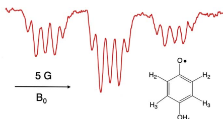
Fig. 1 X-band TREPR spectrum acquired 1 \mu\text{s} after a 10 ns, 355 nm laser pulse firing on the PCET system shown in Scheme 1 (150 \mu\text{L} \text{Ru(III)bpz}(\text{bpy})_2\text{PF}_6 , 0.1 M HQ). The spectrum was collected in dry acetonitrile at room temperature, and is assigned to the \text{HQ}^\bullet structure shown. Hyperfine coupling constants are as follows: \text{H}_2 ( ortho , 5.66 Gauss, triplet), \text{H}_3 ( meta , 0.72 Gauss, triplet), \text{OH}_1 (1.62 Gauss, doublet).
