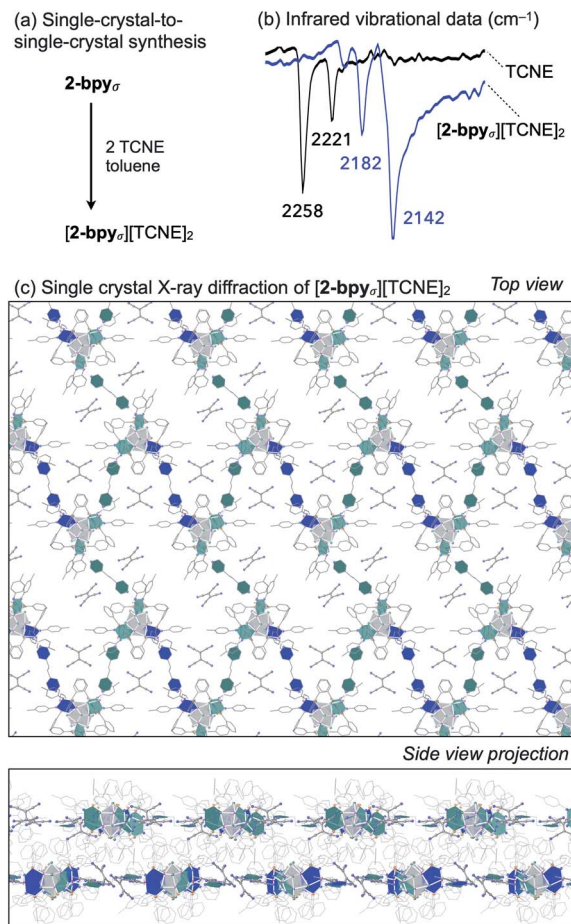
Fig. 6 (a) Single-crystal-to-single-crystal synthesis of [2- bpy σ ][TCNE] 2 via redox intercalation. (b) ATR-FTIR analysis of [2- bpy σ ][TCNE] 2 and TCNE, highlighting the CN stretching region. (c) Single crystal X-ray structure of [2- bpy σ ][TCNE] 2 (top and side views).
