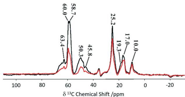
Fig. 13 ^{13}\text{C} spectra observed with (S, black) and without ( S_0 , red) \{^{27}\text{Al}\} S-RSPDOR for the trapped products retained in H-ZSM-5 after reaction with methanol for 15 minutes at 573 K. NMR spectra obtained at a MAS rate of \nu_r = 10 kHz. Reprinted (adapted) with permission from ref. 74. Copyright 2017 American Chemical Society.
