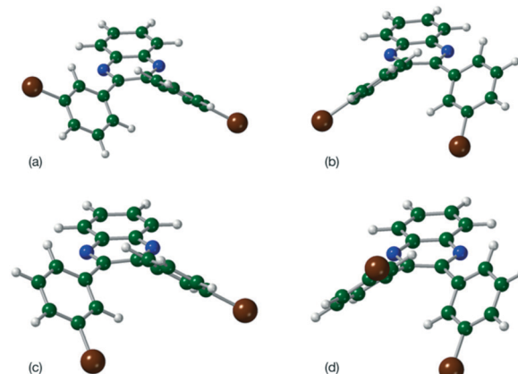
Fig. 2 Molecular geometries for the four located minima of Q3,3'Br 2 (a) \tau_1, \tau_2 = -41^\circ, -41^\circ (b) \tau_1, \tau_2 = 41^\circ, -136^\circ (c) \tau_1, \tau_2 = 136^\circ, -41^\circ and (d) \tau_1, \tau_2 = -136^\circ, 41^\circ .
