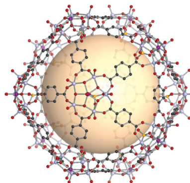
Fig. 22 Structural illustration of [\text{WV}_5\text{O}_{11}\text{SO}_4]_{12}(\mathbf{A1})_{30} . 86
