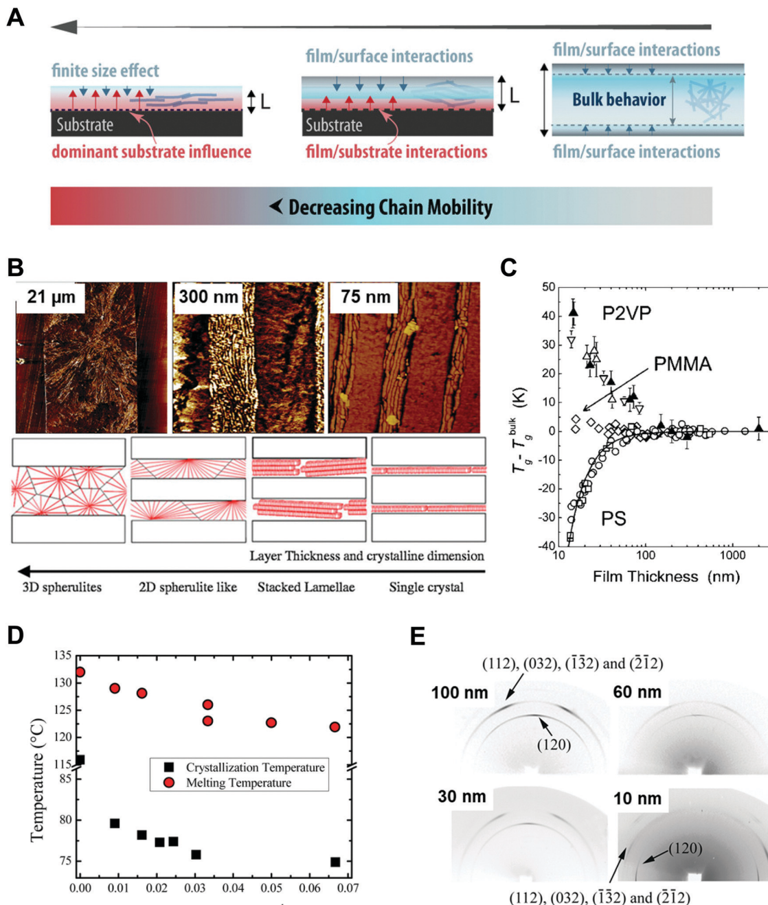
Fig. 4 (A) Schematic illustration of bilayer model to explain nano-confinement effect on polymers. Adapted from ref. 81 with permission from American Chemical Society, copyright 2018. (B) AFM phase images of PS/PEO layered films with different thickness and schematic illustration showing morphology changes of PS/PEO films depending on film thickness. Adapted from ref. 82 with permission from American Chemical Society, copyright 2018 and from ref. 84 with permission from Material Research Science, copyright 2012. (C) T_g - T_g^{\text{bulk}} of PS film, PMMA film and P2VP film as a function of film thickness. Adapted from ref. 80 with permission from American Chemical Society, copyright 2007. (D) Crystallization temperature and melting temperature of PE infiltrated in AAO templates as a function of the inverse of the pore diameter of AAO. Adapted from ref. 14 with permission from John Wiley and Sons, copyright 2014. (E) Wide-angle X-ray diffraction (WAXD) 2D patterns of PEO infiltrated in AAO with different pore sizes. Adapted from ref. 90 with permission from American Chemical Society, copyright 2013.
