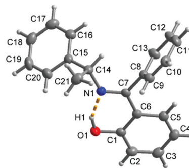
Fig. 3 Molecular structure of R\text{-HL}^1 with the dashed orange line showing the intramolecular hydrogen bond with O1–H1 0.91(2) Å, H1...N1 1.70(3) Å, O1...N1 2.533(2) Å, O1–H1...N1 angle 151(2)^\circ .
