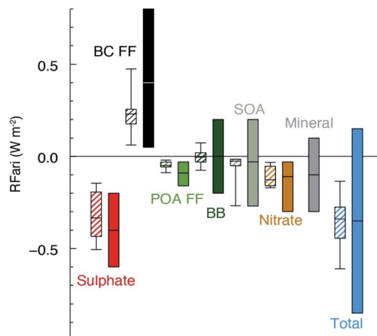
Fig. 1 Annual mean top of the atmosphere radiative forcing due to aerosol–radiation interactions (RF ari , in \text{W m}^{-2} ) due to different anthropogenic aerosol types, for the 1750–2010 period. Hatched whisker boxes show median (line), 5th to 95th percentile ranges (box) and min/max values (whiskers) from AeroCom II models 43 corrected for the 1750–2010 period. Solid coloured boxes show the IPCC Assessment Report 5 (AR5) best estimates and 90% uncertainty ranges. BC FF is for black carbon from the fossil fuel (FF) and the biofuel, POA FF is for primary organic aerosol from fossil fuel and biofuel, BB is short for BBOA for biomass burning organic aerosols and SOA is for secondary organic aerosol. The figure and the caption were reproduced from ref. 1 with permission from Cambridge University Press, © 2013.
