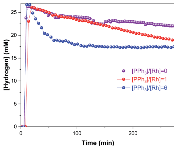
Fig. 9 Hydrogen concentration profiles during [\text{Rh}(\text{CO})_2(\text{acac})] + \text{PPh}_3 catalysed hydroformylation of 1-hexene in toluene at 50 °C and 12 bar of \text{H}_2/\text{CO} (1 : 1) monitored using operando ^1\text{H} FlowNMR spectroscopy. [\text{Rh}(\text{CO})_2(\text{acac})] = 2.5 \text{ mM} , [1\text{-hexene}] = 500 \text{ mM} , [\text{PPh}_3] varied as indicated.
