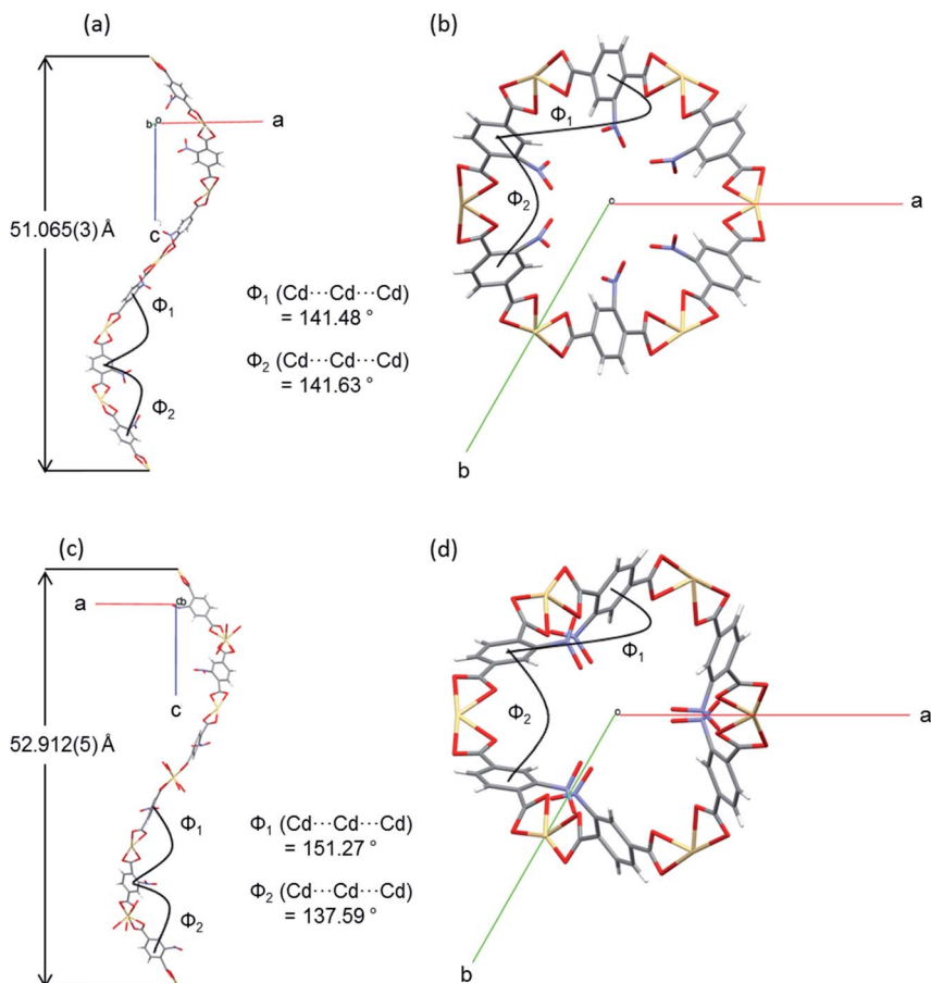
Fig. 4 A single turn of a helix viewed perpendicular and parallel to the c -axis, along which the helices and accompanying pores propagate, shown with dimensions for alternating \text{Cd} \cdots \text{Cd} \cdots \text{Cd} angles ( \phi_1 , \phi_2 ) and the helix pitch, for (a) and (b) SHF-81-DMF; (c) and (d) SHF-81. Single-crystal structures determined at 100 K.
