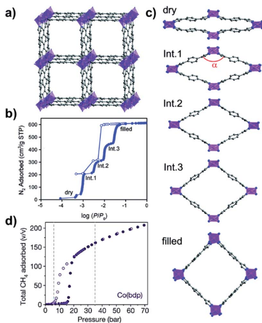
Fig. 14 (a) Crystal structure of as-synthesised Co(bdp); (b) \text{N}_2 sorption isotherms of Co(bdp)-dry at 77 K; (c) phase transition during \text{N}_2 sorption; and (d) \text{CH}_4 sorption isotherms of Co(bdp)-dry at 298 K. Reproduced from ref. 74 and 102 with permission; copyrights: 2015, Springer Nature and 2010, American Chemical Society.
