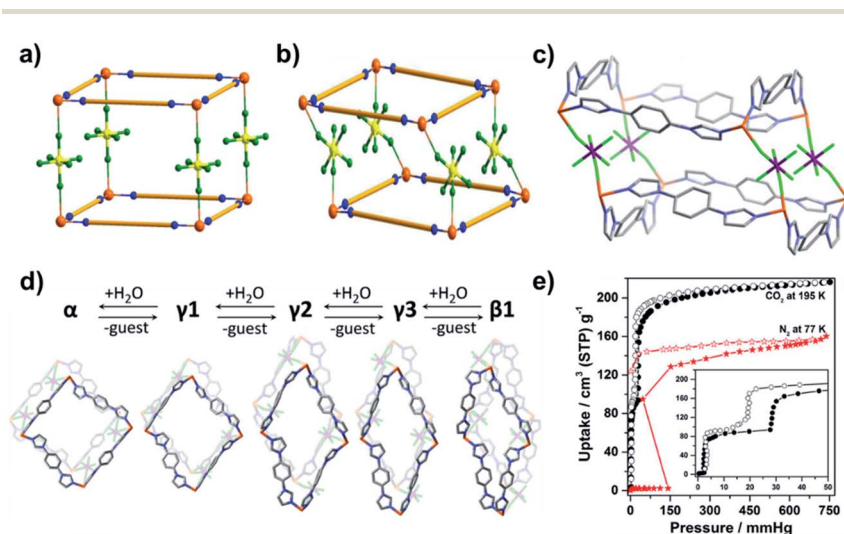
Fig. 12 Schematic diagrams of (a) traditional SIFSIX- n -M networks with trans -bridging SIFSIX pillars and (b) SIFSIX-23-Cu with cis -bridging SIFSIX pillars; (c) coordination mode and geometry in SIFSIX-23-Cu; (d) reversible structural transformations in SIFSIX-23-Cu; (e) \text{N}_2 (77 K) and \text{CO}_2 (195 K) sorption isotherms of SIFSIX-23-Cu. Reproduced from ref. 151 with permission; copyright: 2020, American Chemical Society.
