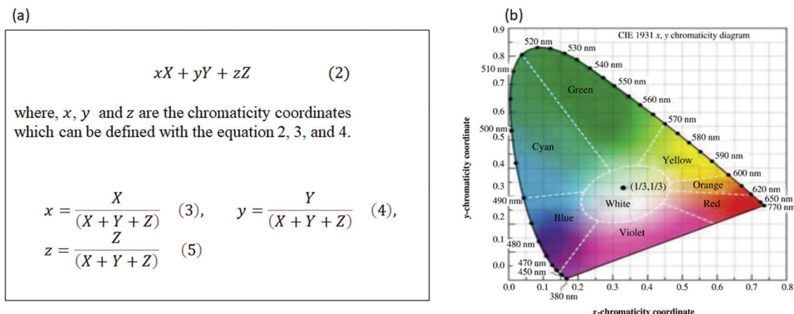
Fig. 4 (a) Equations to calculate the color space coordinates, (b) Chromaticity diagram CIE 1931 in 2-dimension plane (reprinted with permission from the ref. 70).
