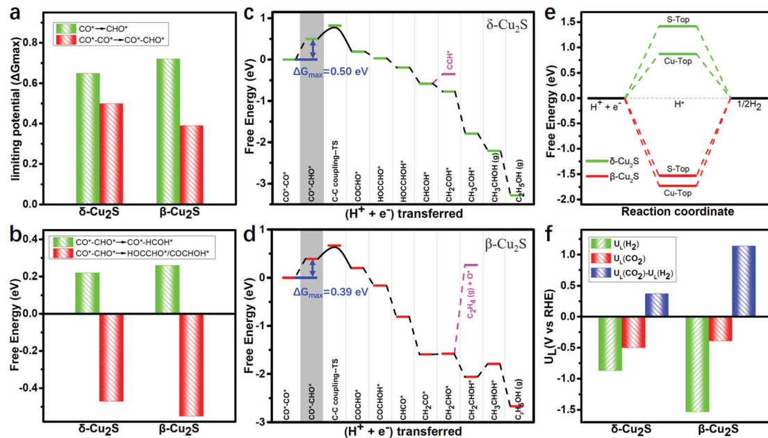
Fig. 3 Free energy of the hydrogenation step of (a) \text{CO}^* \rightarrow \text{CHO}^* and \text{CO}^* \rightarrow \text{CO}^* , (b) \text{CO}^* \rightarrow \text{CHO}^* and \text{CO}^* \rightarrow \text{CO}^* to \text{HOCCHO}^*/\text{COCHOH}^* . Free energy diagrams of \text{CO}^* \rightarrow \text{CO}^* hydrogenation to \text{C}_2\text{H}_5\text{OH} on (c) \delta\text{-Cu}_2\text{S} and (d) \beta\text{-Cu}_2\text{S} . Limiting potential is obtained from the maximum free energy change ( \Delta G_{\text{max}} ) of the whole reaction process, which is marked by blue lines. (e) Free energy profiles of the HER on \delta\text{-Cu}_2\text{S} (green line) and \beta\text{-Cu}_2\text{S} (red line). (f) Limiting potentials for the \text{CO}_2\text{RR} U_L(\text{CO}_2) , HER U_L(\text{H}_2) and difference U_L(\text{CO}_2) - U_L(\text{H}_2) on \delta\text{-Cu}_2\text{S} and \beta\text{-Cu}_2\text{S} monolayers.
