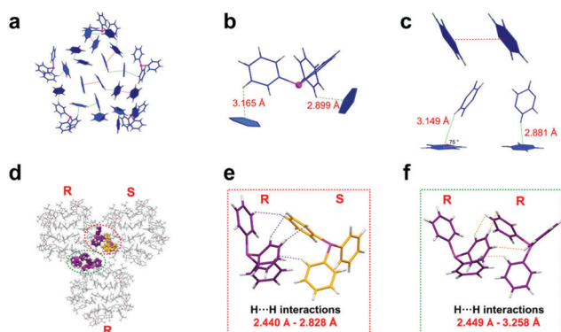
Fig. 4 (a) The interactions of Ag 70 -TPP surface ligands; (b) the intra-molecular C–H··· \pi interaction; (c) the C–H··· \pi interaction and \pi ··· \pi stacking; (d) interaction of adjacent clusters in the lattice; (e) H···H interactions of the cluster with opposite chirality; (f) H···H interactions of the cluster with the same chirality.
