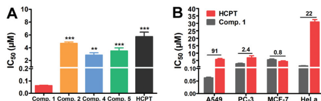
Fig. 3 Cytotoxicity of the tandem self-assembling prodrug. (A) \text{IC}_{50} value of A549 cells treated with Comp. 1 , 2, 4, 5 and free HCPT. (B) \text{IC}_{50} value of Comp. 1 and HCPT to different cell lines. (One-way ANOVA, compared to the Comp. 1 group, mean \pm SD, *** P < 0.001, ** P < 0.01. N = 3.)
