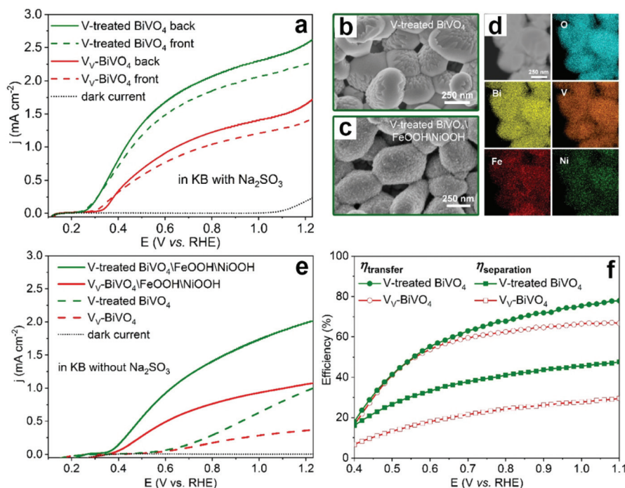
Fig. 8 (a) Photocurrent density versus applied potential curves of the \text{BiVO}_4 with vanadium vacancies ( \text{V}_\text{V}\text{-BiVO}_4 ) and V-treated \text{BiVO}_4 photoanodes. SEM images of V-treated \text{BiVO}_4 (b) before and (c) after the deposition of \text{FeOOH/NiOOH} cocatalysts. (d) STEM image and elemental mapping of O, Bi, V, Fe and Ni for V-treated \text{BiVO}_4 . (e) Photocurrent density versus applied potential curves of \text{V}_\text{V}\text{-BiVO}_4 and V-treated \text{BiVO}_4 with and without \text{FeOOH/NiOOH} cocatalysts. (f) Charge-transfer and charge-separation efficiencies versus applied potential curves of \text{V}_\text{V}\text{-BiVO}_4 and V-treated \text{BiVO}_4 photoanodes. Reproduced from ref. 99 with permission. Copyright 2021, American Chemical Society.
