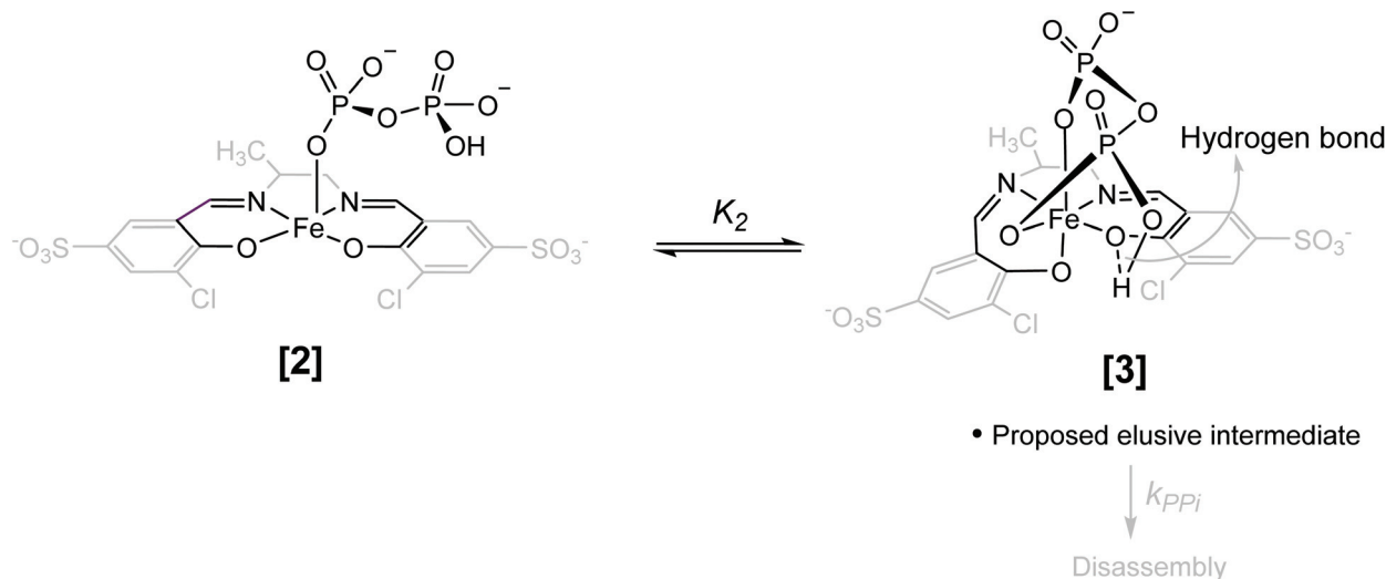
Scheme 2 “Induced fit” linkage isomerism of complex 1\text{-OP(O)}_2\text{OPO}_2(\text{OH})_2^{2-} deduced from mechanistic studies. A hypothesized octahedral elusive intermediate [3] is also depicted which was supported by computational studies.
