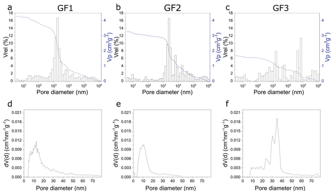
Fig. 3 Pore width distributions of samples GF1, GF2 and GF3 obtained using Hg intrusion (a–c), and \text{N}_2 sorption (d–f).
