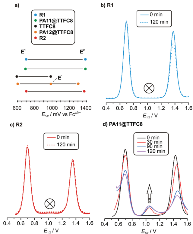
Fig. 8 Electrochemical data: (a) Correlation diagram of DPV peak potentials of all relevant (pseudo)rotaxane species, DPVs before and after electrolysis of (b) R1 , (c) R2 , (d) PA11@TTFC8 ( CH_2Cl_2 , with n-Bu_4NBARF_{24} as the electrolyte (0.1 M), 298 K, 1 mM analyte, 25 mV modulation amplitude, 50 ms modulation time, 5 mV step potential, 0.5 s interval time).
