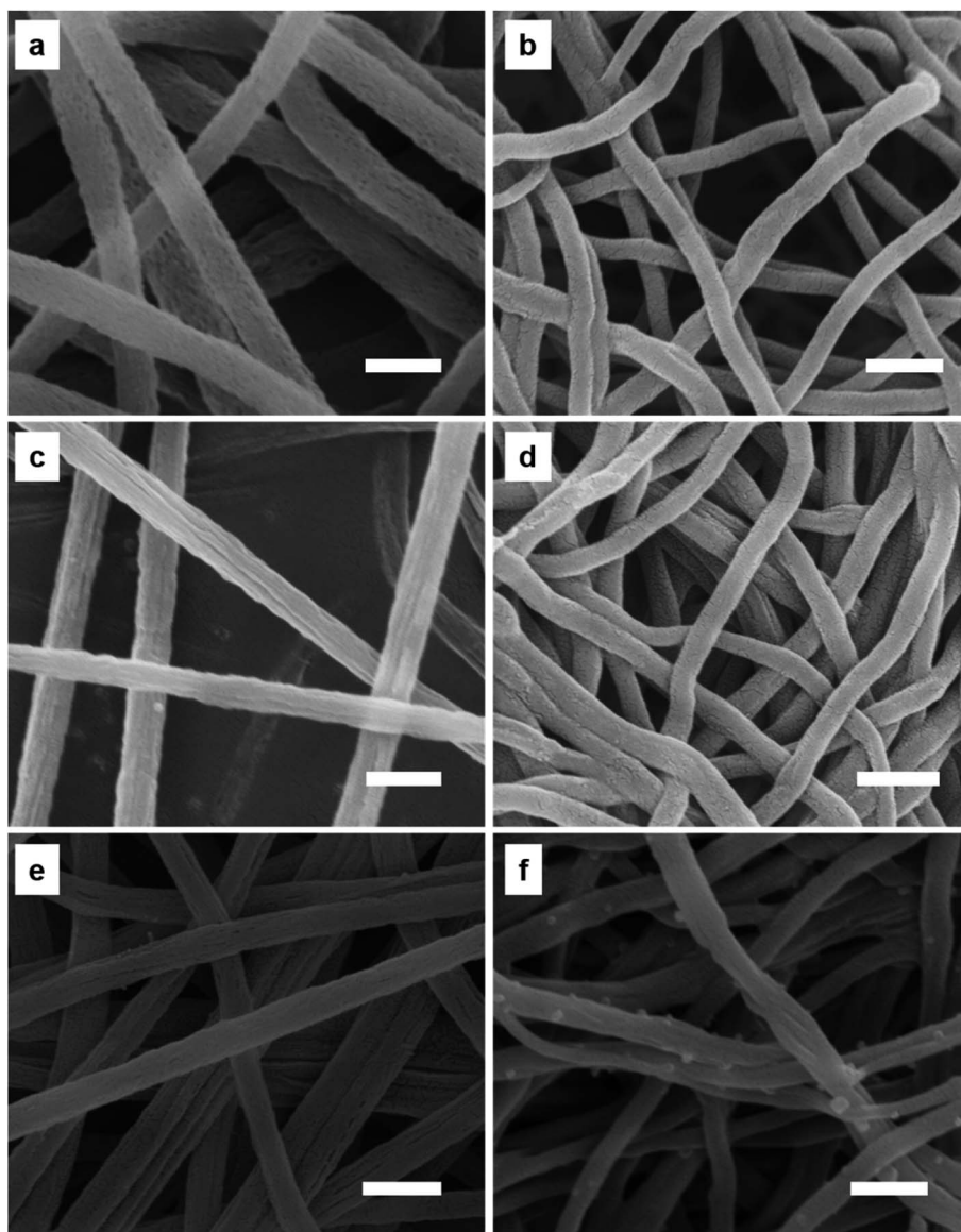
Fig. 4 SEM images of (a) porous PAN, (b) PCNFs, (c) porous PAN/PFSA, (d) 0.1F-PCNFs, (e) 0.1Li-porous PAN/PFSA, and (f) 0.1Li-PCNFs composites. The scale bar is 500 nm.
