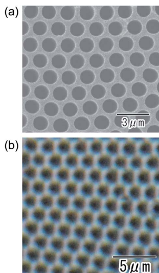
Fig. 7 SEM (a) and optical microscope (b) images of highly ordered porous alumina obtained at 700 V. The anodization was carried out in an electrolyte with a mixture of water and tetraethylene glycol (1 : 1 volume ratio) containing 25 mM citric acid and 0.25 mM phosphoric acid at 16 °C for 550 h. The thickness of the sample was 280 μm.
