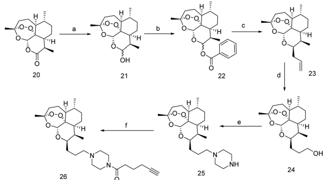
Scheme 4 (a) NaBH 4 , MeOH, 0 °C; (b) benzoyl chloride, pyridine, DMAP, CH 2 Cl 2 , rt; (c) AllylTMS, ZnCl 2 , 0 °C.; (d) (1) BH 3 ·SMe 2 , Et 2 O, -20 °C.; (2) H 2 O 2 , Na 2 CO 3 , H 2 O, rt; (e) (1) MsCl, Et 3 N; (2) piperazine, THF, reflux; (f) 5-hexanoic acid, EDCI, HOBt, dry DCM, rt (97%).
