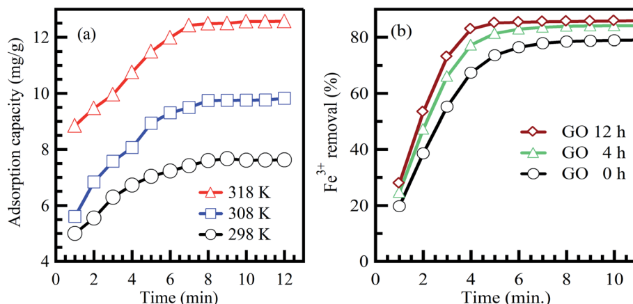
Fig. 4 Effect of contact time on the adsorption of (a) bromothymol blue dye on polyvinyl alcohol adsorbent, adapted with permission from ref. 49, copyright, Elsevier, 2016, and (b) \text{Fe}^{3+} on graphene oxide aerogel adsorbent, adapted with permission from ref. 50, copyright, Elsevier, 2019.
