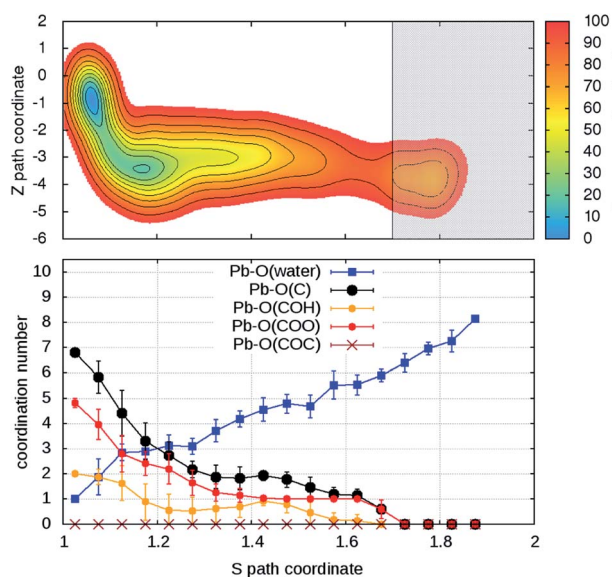
Fig. 4 (Upper panel) Free energy surface for the unbinding of Pb reconstructed from one out of two (Fig. S6†) independent ab initio metadynamics simulations in different environments. The shaded area ( S > 1.7 ) represents the region where the bias profile is not representative of the free energy, due to lack of reverse transition (binding). (Lower panel) Evolution of the coordination numbers of Pb and O belonging to water and to different organic functional groups, as a function of the S path coordinate. The vertical bars represent standard deviations of coordination numbers.
