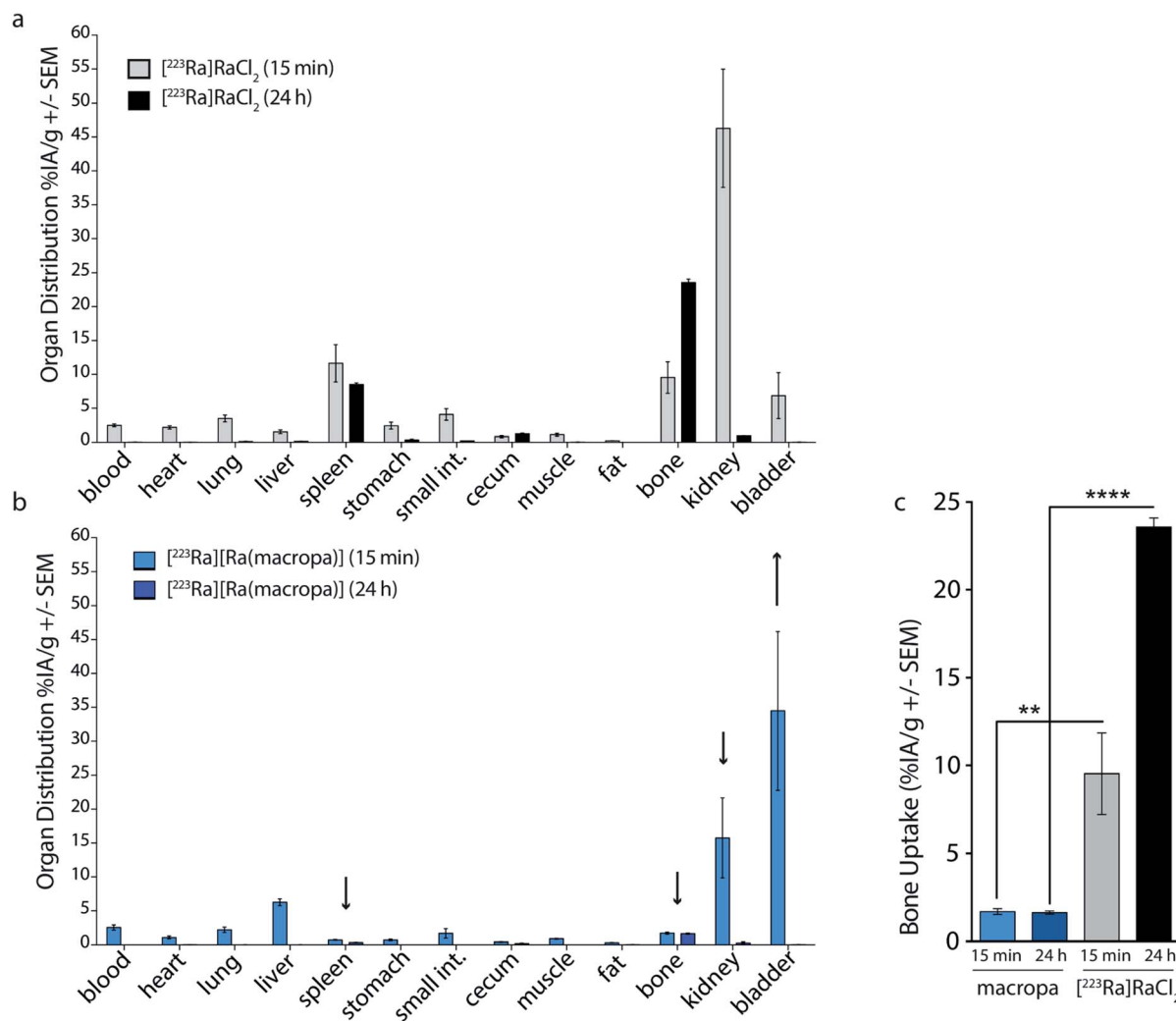
Fig. 4 In vivo evaluation of ^{223}\text{Ra} [Ra(macropa)]. (a) ^{223}\text{Ra} Cl 2 and (b) ^{223}\text{Ra} [Ra(macropa)] radioactive organ distribution (% injected activity normalized to weight; % IA per g) was assessed utilizing healthy, skeletally mature mice sacrificed at 15 min and 24 h p.i. Differences in splenic, renal, and bone uptake were observed between the two groups. (c) Mice administered ^{223}\text{Ra} [Ra(macropa)] exhibited 10 to 25-fold lower osseous uptake than that of free ^{223}\text{Ra} at 15 min and 24 h p.i. (** p = 0.0096; **** p < 0.0001).
