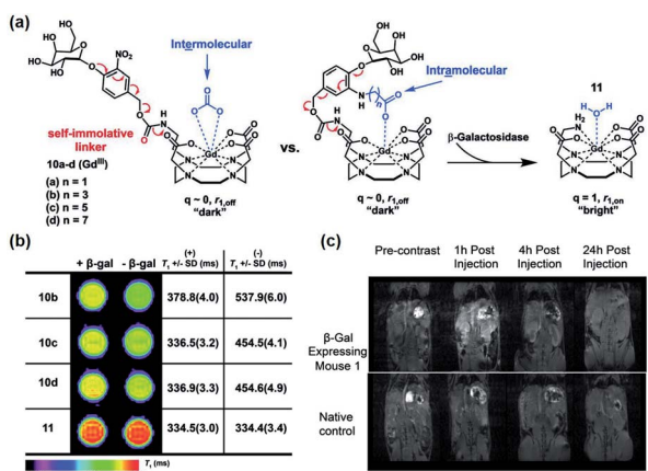
Fig. 10 (a) Self-immolative MRI contrast agents with intermolecular or intramolecular architecture for \beta -gal detection. (b) MR information of (10b–d) \pm\beta -gal at 7 T. (c) MR images of living mice.
