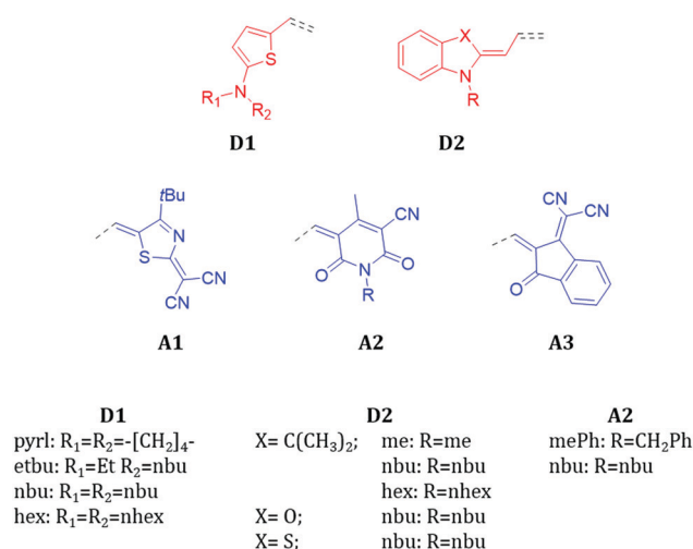
Fig. 1 Molecular structures of the donor and acceptor units constituting the library of merocyanines investigated in the current work. Details of the various side chains and heteroatoms characterising the D and A units are reported at the bottom.
