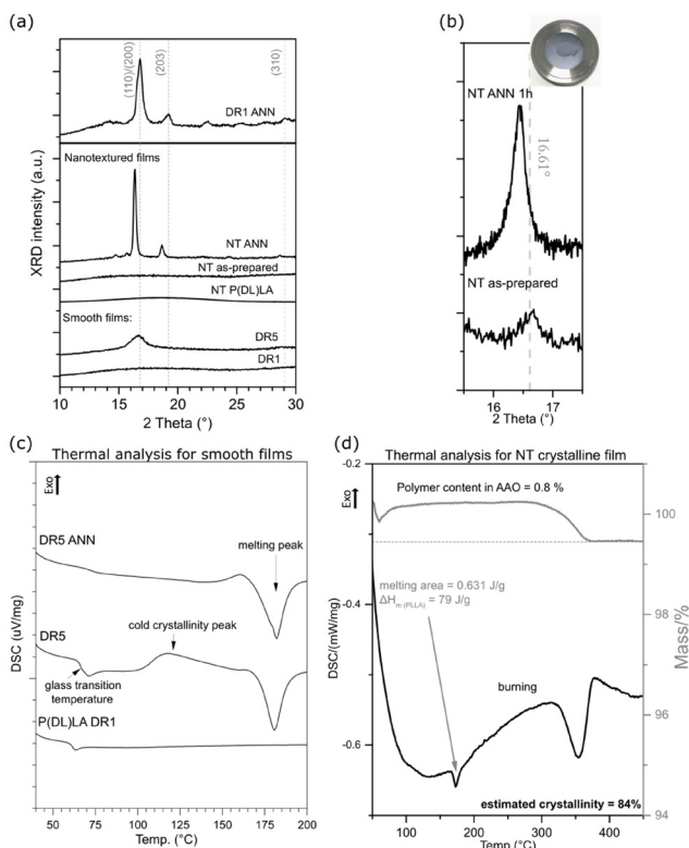
Fig. 3 (a) XRD diffractograms of nanotextured films (NT as-prepared, annealed (NT ANN) at 160 °C for 1 h and for P(DL)LA as-prepared (NT P(DL)LA)) and smooth films (non-drawn (DR1) and drawn (DR5) compared to unoriented annealed film (DR1 ANN) at 160 °C for 1 h. (b) XRD of mechanically extracted nanotubes for NT as-prepared and NT ANN tubes. Thermal analysis (DSC and mass lost) of (c) drawn films (DR5, DR5 ANN and P(DL)LA DR1) and (d) filled AAO template with polymer excess ground off on the bottom of the NT ANN sample.
