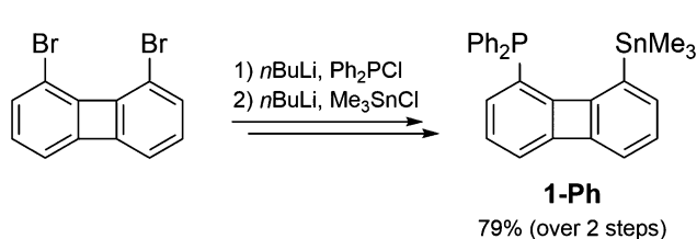
Scheme 1 Synthesis of the precursor for an Al-Sn exchange 1-Ph .
