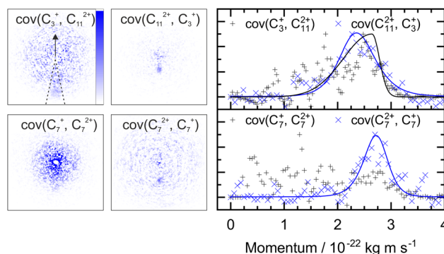
Fig. 4 Left: The covariance map images for dissociation of PHE 3+ into \text{C}_3\text{H}_x^+ and \text{C}_{11}\text{H}_y^{2+} , and \text{C}_7\text{H}_x^+ and \text{C}_7\text{H}_y^{2+} , top and bottom, respectively. Nomenclature as in Fig. 2. Covariance signal in the \text{cov}(\text{C}_7^+, \text{C}_7^{2+}) image cannot be discerned above the noise level but the \text{cov}(\text{C}_7^{2+}, \text{C}_7^+) image provides the TKER for the dissociation process. The centre of the \text{cov}(\text{C}_7\text{H}_x^+, \text{C}_7\text{H}_y^{2+}) image shows detector saturation due to the flight times of \text{C}_7\text{H}_x^+ and \text{C}_{14}\text{H}_y^{2+} overlapping. Right: the momentum profiles extracted from the corresponding covariance images using the region marked by dashed lines in the \text{cov}(\text{C}_3^+, \text{C}_{11}^{2+}) image. All images and momentum profiles are individually normalized.
