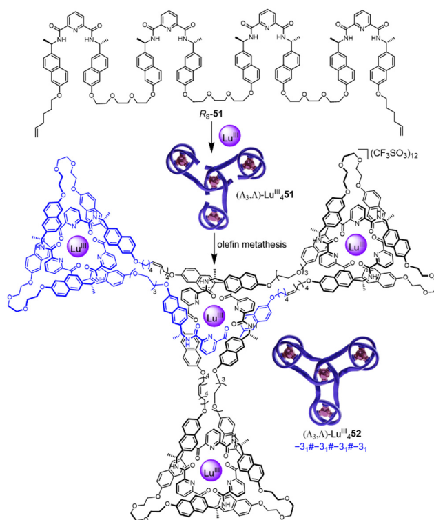
Fig. 18 Synthesis of triskelion knot (\Lambda_3, \Lambda)\text{-Lu}_4^{\text{III}}\mathbf{52} by Vernier template synthesis. 27
