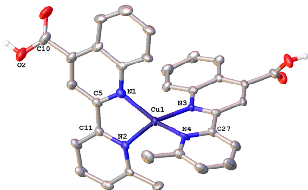
Fig. 5 Molecular structure of the cation of complex 2[\text{Cu}(6'\text{-Mepqca})_2][\text{PF}_6] \cdot \text{Me}_2\text{CO} \cdot 0.5\text{H}_2\text{O} ( 2(2\text{-Me}_2\text{CO} \cdot 0.5\text{H}_2\text{O}) ); ellipsoids are plotted at the 50% probability level. H atoms, except those in the COOH groups, and the co-crystallized solvents are omitted for clarity.
