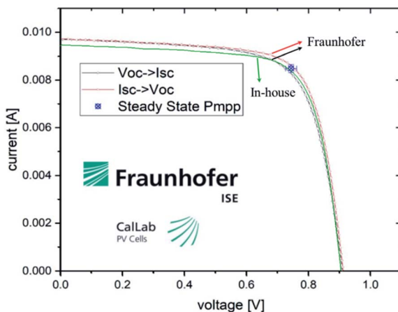
Fig. 3 \text{Cu(In,Ga)S}_2/(\text{Zn,Sn)O/Al:ZnMgO/Al:ZnO} certified I - V curves of the 14.0% efficiency device measured at the Fraunhofer Institute for Solar Energy Systems. The red curve is the measurement from the short-circuit current to the external open-circuit voltage, and the black curve is the measurement from the external open-circuit voltage to the short-circuit current. The olive curve is the in-house measurement. The blue square point shows the steady-state maximum power-point of the device achieved by keeping the device at V_{\text{mpp}} for 5 minutes.
