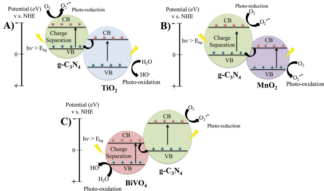
Fig. 6 Schematic of band structures and charge transfer mechanism in direct Z-scheme heterojunction structures: (A) \text{g-C}_3\text{N}_4\text{-TiO}_2 ; (B) \text{g-C}_3\text{N}_4/\text{MnO}_2 ; and (C) \text{TBiVO}_4/\text{g-C}_3\text{N}_4 .
