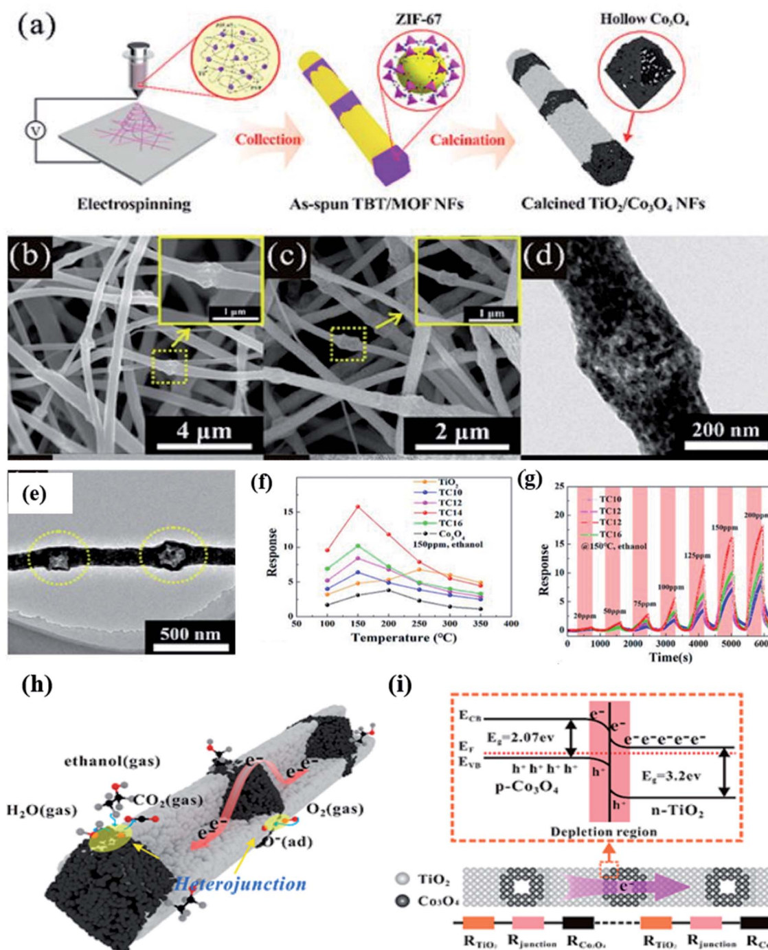
Fig. 8 (a) Schematic diagram of the fabrication procedure of MOF derived Co 3 O 4 -TiO 2 NFs, (b-e) SEM and TEM images of TiO 2 -Co 3 O 4 NFs, (f) response versus temperature study of TiO 2 -Co 3 O 4 NFs, (g) ethanol response transients of the TiO 2 -Co 3 O 4 NF sensor at 150 °C, (h and i) gas sensing mechanism of the TiO 2 -Co 3 O 4 NF sensor along with the corresponding energy band diagram of the TiO 2 -Co 3 O 4 NF sensor. Reproduced from ref. 96, copyright@2021, American Chemical Society.
