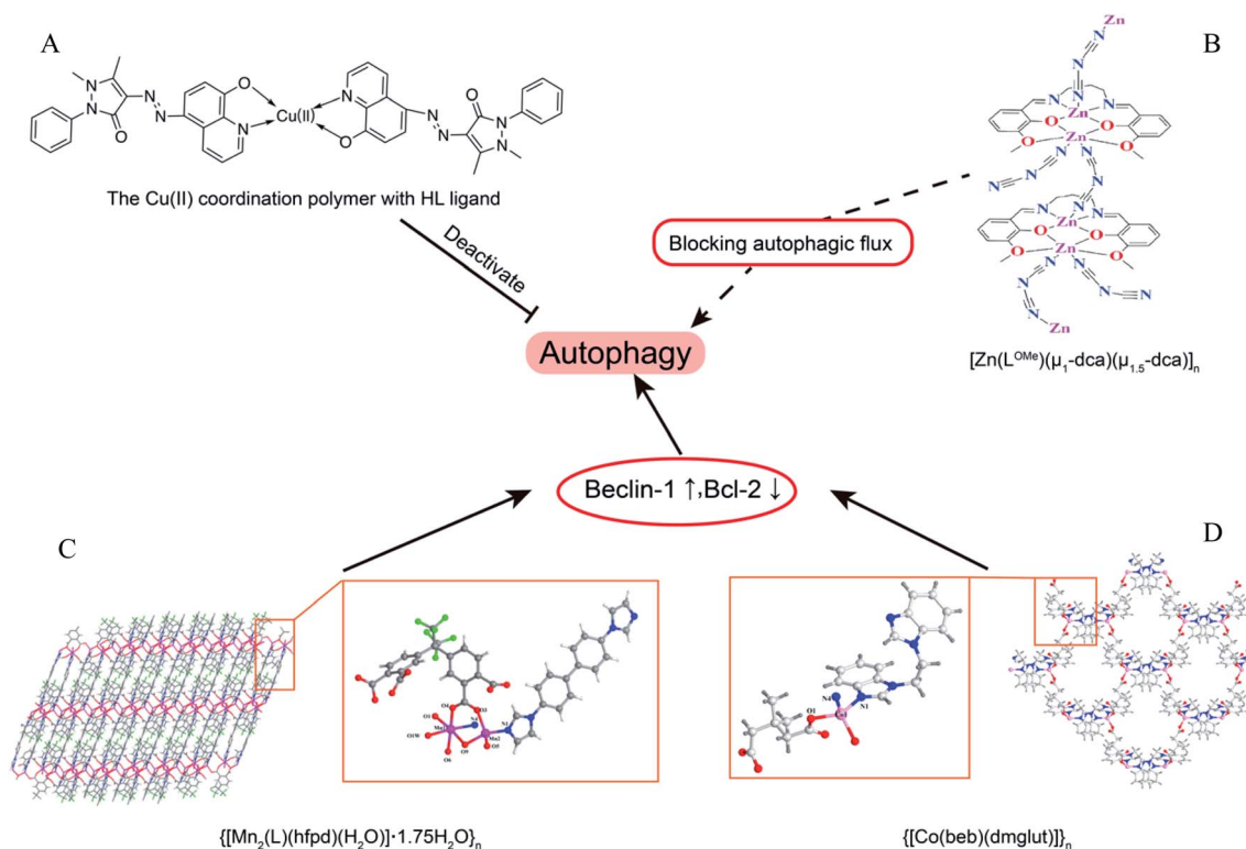
Fig. 6 The overview of coordination polymers affecting autophagy. (A) Chemical structure of Cu(II) coordination polymer with HL ligand. 82 (B) Zn(II) coordination polymer, [Zn(L OMe )(μ 1 -dca)(μ 1.5 -dca)] n , blocked autophagic flux. The asymmetry unit views and skeleton structures for (C) [Mn 2 (L)(hfpd)(H 2 O)] n · 1.75H 2 O (ref. 81) and (D) [Co(beb)(dmglut)] n , 83 which induce autophagy via regulating Beclin1 and BCL-2.
