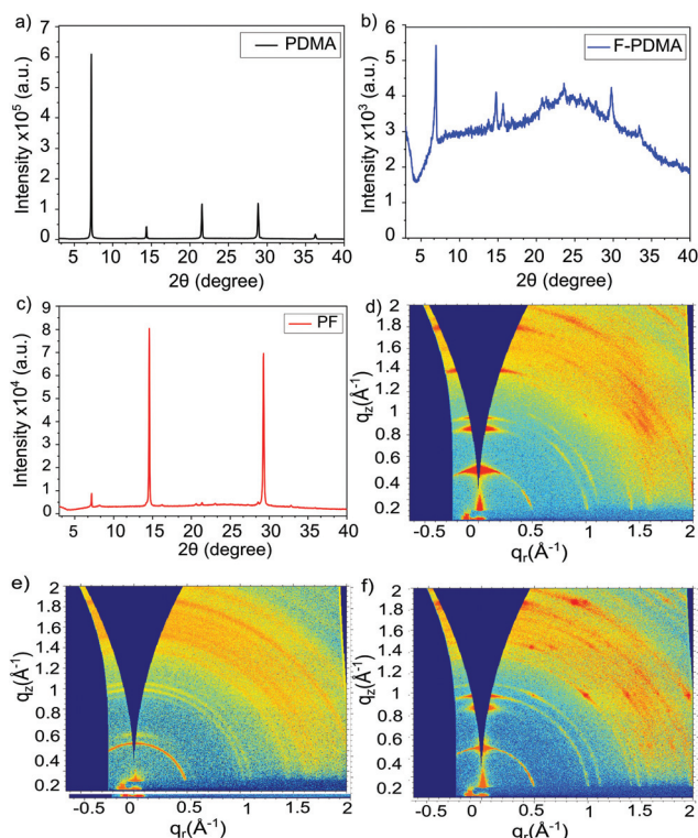
Fig. 2 Structural properties of layered hybrid perovskites. (a–c) XRD patterns of thin films based on (a) (\text{PDMA})\text{PbI}_4 (black), (b) (\text{F-PDMA})\text{PbI}_4 (blue), and (c) (\text{PF})\text{PbI}_4 (red) compositions on microscope glass. (d–f) GIWAXS patterns of thin films of (d) (\text{PDMA})\text{PbI}_4 , (e) (\text{F-PDMA})\text{PbI}_4 , and (f) (\text{PF})\text{PbI}_4 . Methods and further analysis is provided in the ESI. †
