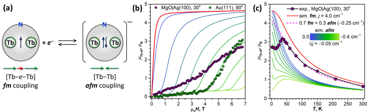
Fig. 10 (a) Schematic description of the electron trapping by the SOMO of Tb_2@C_{79}N leading to Tb_2@C_{79}N^- anion with two-fold occupied Tb\text{-}4f bonding MO and antiferromagnetic coupling of magnetic moments; green arrows denote Tb\text{-}4f magnetic moments, red arrow denotes magnetic moment of the unpaired valence electron. (b) Magnetization curves of Tb_2@C_{79}N on MgO|Ag(100) and Au(111) measured at T \approx 2 \text{ K} and compared to the results of simulations for fm and afm coupling of Tb\text{-}4f magnetic moments, the coloring scheme is the same as in (c). (c) Temperature dependence of Tb\text{-}4f magnetic moment in Tb_2@C_{79}N 1.5 ML on MgO|Ag(100) measured by XMCD at 6.8 T in grazing incidence and compared to the results of simulations for ferromagnetic (fm) and antiferromagnetic (afm) coupling of Tb\text{-}4f magnetic moments with different values of the coupling constant j_{12} ; dashed line is a simulation for a mixture of molecules with fm (70%) and afm (30%) ground states.
