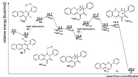
Fig. 9 Relative energy of species in the visible light-induced reaction pathway of 6 with H 2 O 2 . *The relative energy with respect to T1 INT C2P2 was computed for geometries optimized with the def2-SVP basis set.
