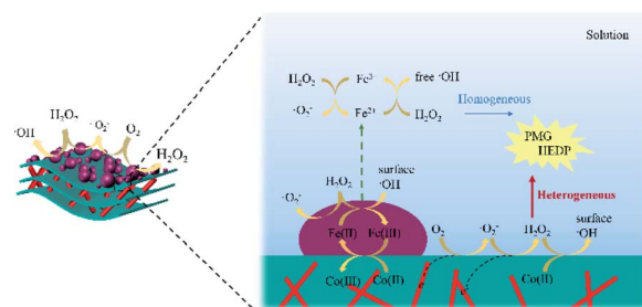
Fig. 12 Possible reaction mechanism of CoNWs@CoAl-LDHs/ \text{Fe}_3\text{O}_4 .
