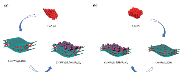
Fig. 11 Synthesis process of CoNWs@CoAl-LDHs/ \text{Fe}_3\text{O}_4 (a) and CoNPs@CoAl-LDHs/ \text{Fe}_3\text{O}_4 (b).
