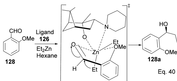
Scheme 34 The transition state in the alkylation of aldehyde 128 mediated by pinene amino alcohol.
