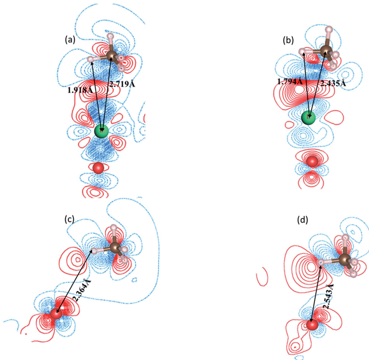
Fig. 3 2-D plots of the calculated electron density difference (EDD) for the CH 4 adsorption. (a) C-H...Ir coplanar on Ir/Fe 2 O 3 (110) surface, (b) C-H...Ir coplanar on Ir/Fe 2 O 3 (110)-O v surface and (c) C-H...O coplanar on Ir/Fe 2 O 3 (110) surface and (d) C-H...O coplanar on Ir/Fe 2 O 3 (110)-O v surface. The red and blue lines represent the increasing and decreasing electron densities, respectively. The isovalue is 0.002 ebohr -3 .
