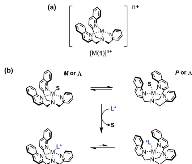
Fig. 1 (a) Structure of [M(\text{BQPA})]^{n+} ; (b) conformational preference induced by displacement of a solvent molecule S from the metal centre by a chiral ligand L^* .
